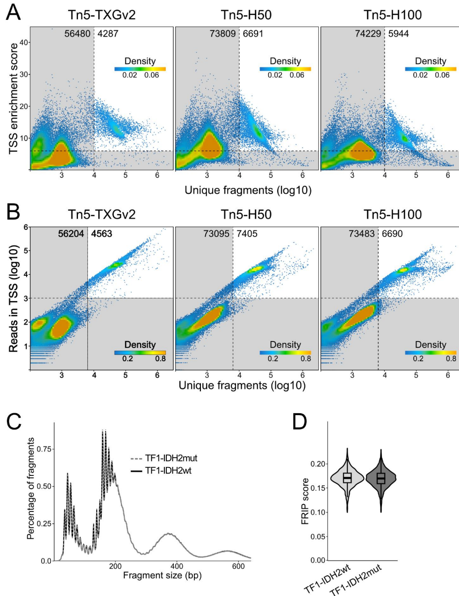
Figure S4. Quality assessment of single cell multiome data. (A) TSS enrichment score over log10 number of unique fragments of cell barcodes in scMultiome-ATAC of PBMCs with the indicated Tn5 preparations. Colors of points reflect density of cell barcodes. Grey area marks low-quality cell barcodes. (B) Same as panel A for log10 number of reads in TSS over log10 number of unique fragments. (C) Fragment size distribution for scMultiome-C&T against H3K27me3 in TF1-IDH2wt and TF1-IDH2mut. (D) Fragments of reads in peaks (FRIP) scores for H3K27me3 per cell in TF1-IDH2wt and TF1-IDH2mut from the scMultiome-C&T analysis.
