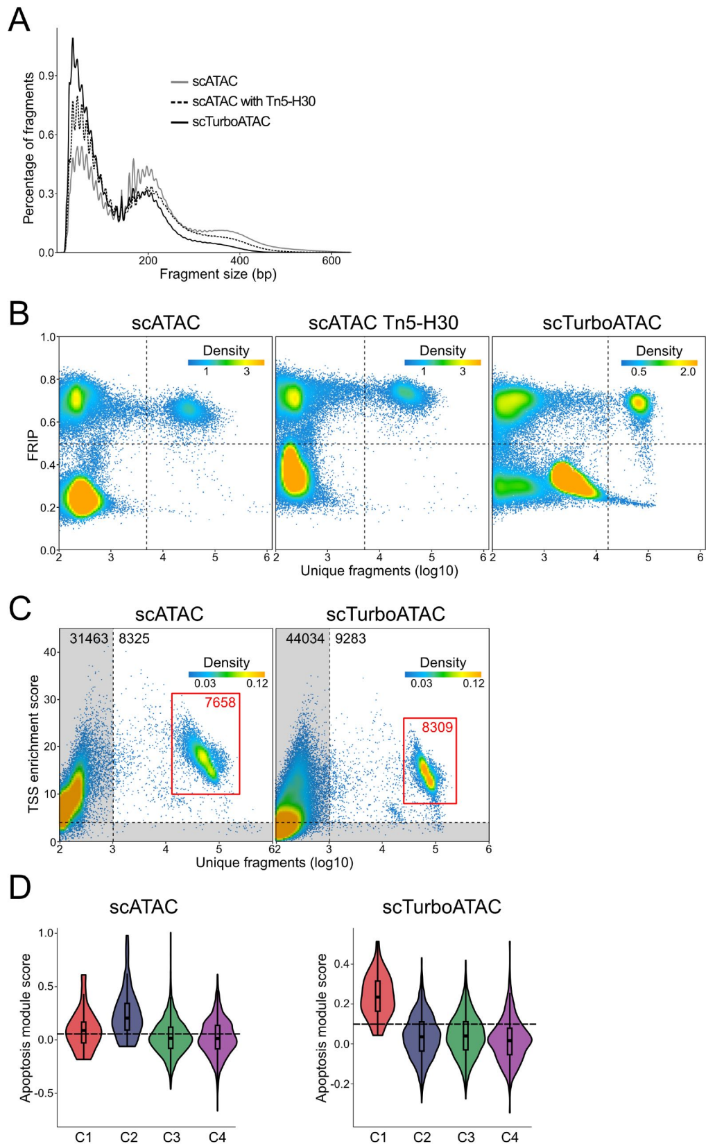
Figure S1. Quality assessment of scTurboATAC data. (A) Fragment size distribution in
