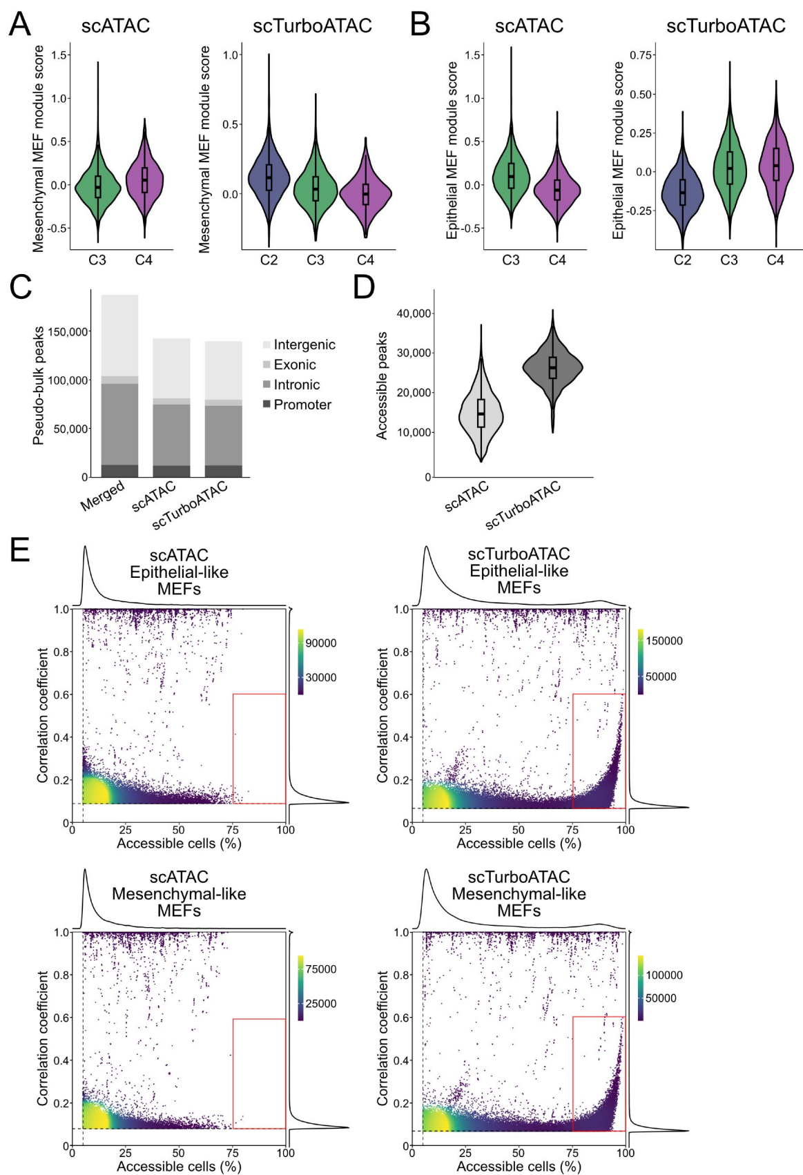
Figure S2. Transcription regulation analysis with scTurboATAC. MEFs stimulated for 6h with IFN \beta were studied. The scATAC data refer to the Tn5-TXGv1.1 enzyme. (A)
